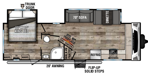
C272FK UVW - 6,780 | Exterior Length - 31'1" | Sleeps - 5
